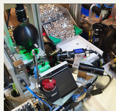
Up to four testing & assembly stations
